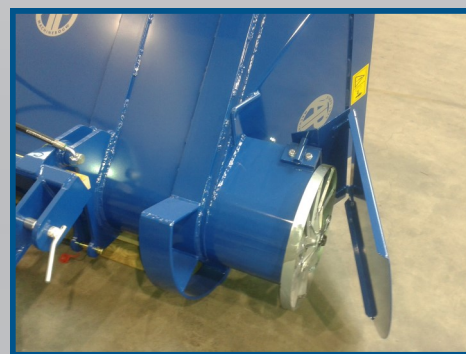
fodder beet cutting device VDCE (8-bladed knife)
